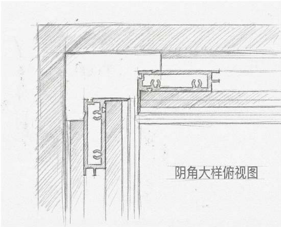
节点Detail
